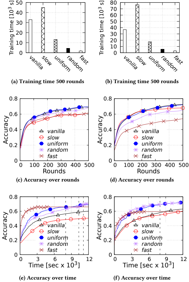
Figure 6: Comparison results for different selection policies on Cifar10 with resource plus non-IID heterogeneity heterogeneity (Column 1) and resource, data quantity, and non-IID heterogeneity heterogeneity (Column 2).
