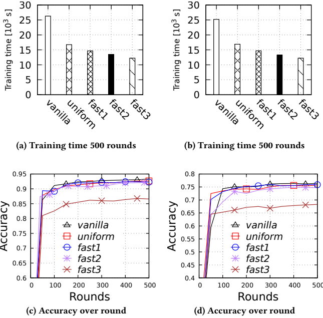
Figure 5: Comparison results for different selection policies on MNIST (Column 1) and FMNIST (Column 2) with resource plus data heterogeneity.
