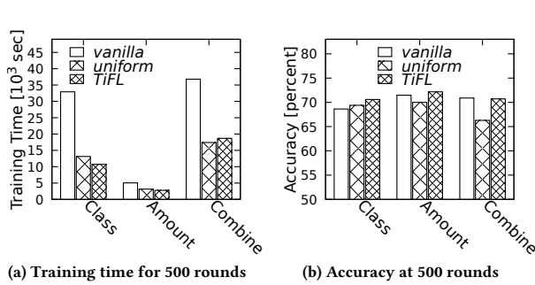
Figure 8: Comparison results for different selection policies on Cifar10 with data quantity heterogeneity (Amount), non-IID heterogeneity (Class), and resource plus data heterogeneity (Combine).
